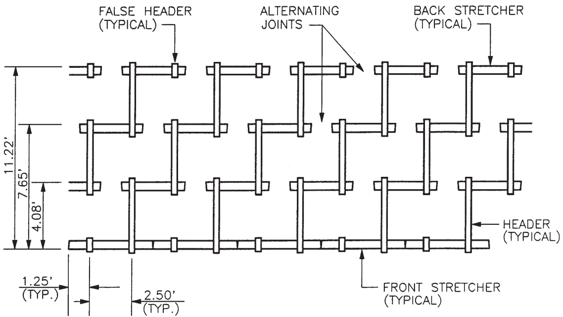
TYPICAL TRIPLE DEPTH PLAN VIEW BASE COURSE 4.5' HEADER
